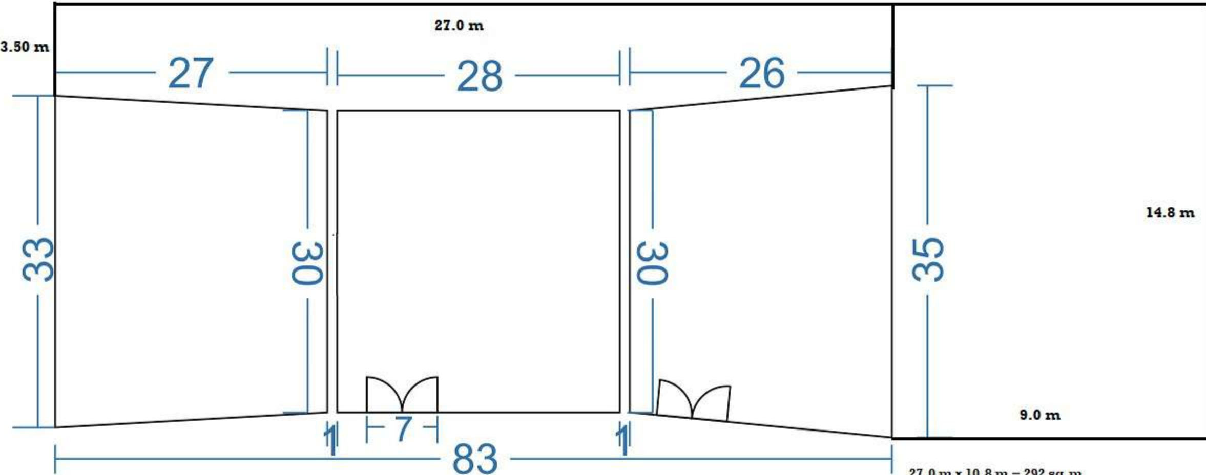
Second Building Ground Floor Plan
